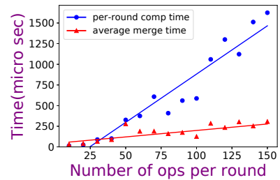
(a) List
