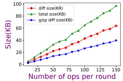
(b) List
