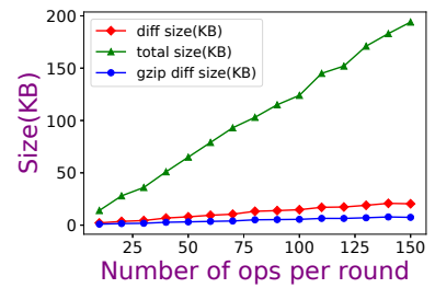
(a) Heap
