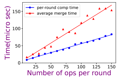
(b) Red-Black Tree
